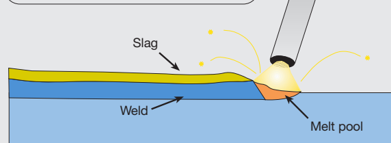
Fig. 1 Shielded Metal-Arc Welding SMAW (MMA)
