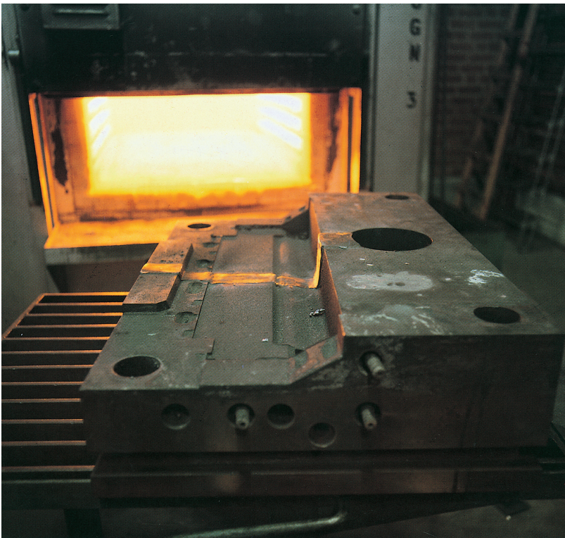
Heat treatment of a die-casting die after welding.
