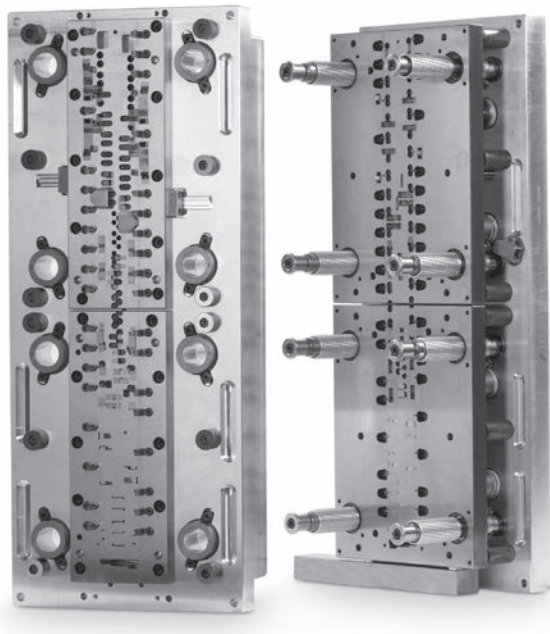
Progressive tool.
