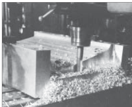
Milling Alumec 89.
