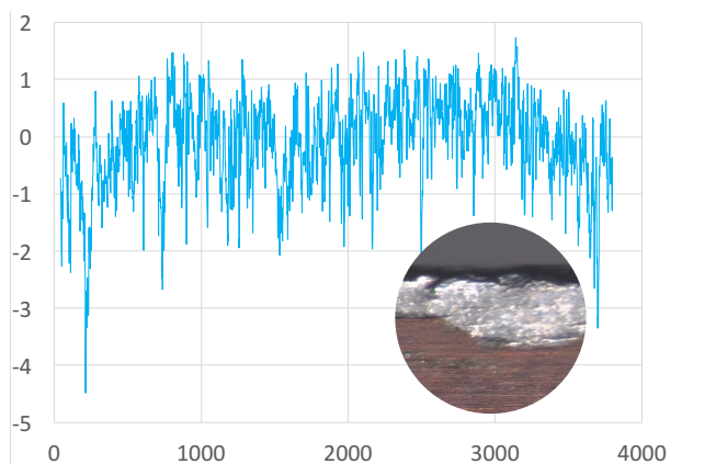
Surface profile with deep grinding marks, R_a = 0,5 \mu\text{m} , R_z = 4,0 \mu\text{m}
