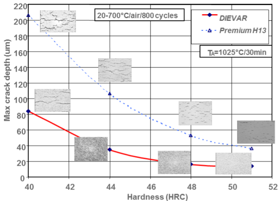
Figure 4 clearly illustrates that Uddeholm Dievar is far superior to premium H13 in solving the industry's biggest problem of heat checking also known as thermal fatigue. If we take the industry standard hardness of 46HRC then Uddeholm Dievar in this test has around 2.5x better resistance to heat checking over premium H13.
