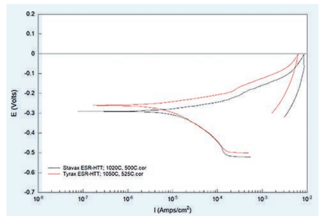
Polarisation curve of Tyrax ESR vs Stavax ESR
