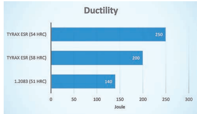
Result from un-notched charpy-v testing.
