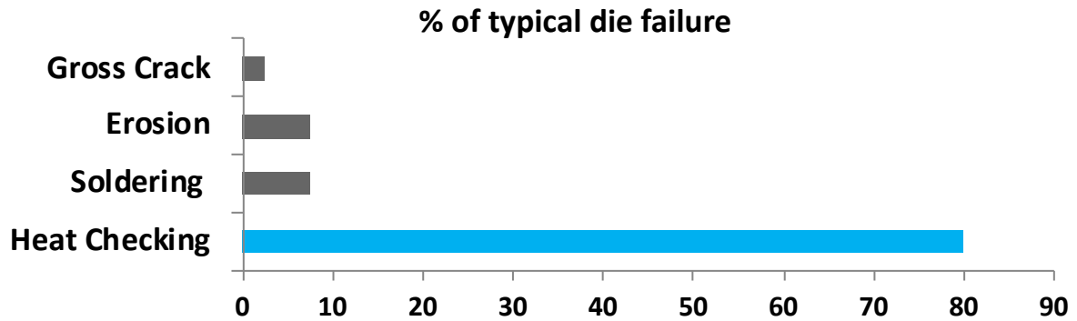
Figure 2 shows the breakdown of typical die failure (percentage) in HPDC
