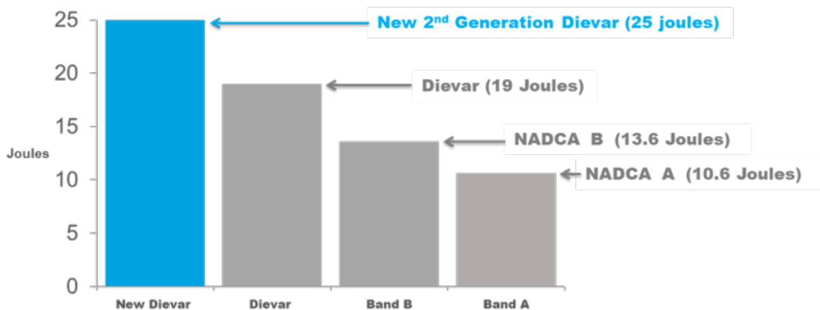
Figure 1 shows the impressive growth of toughness in the new Uddeholm Dievar
