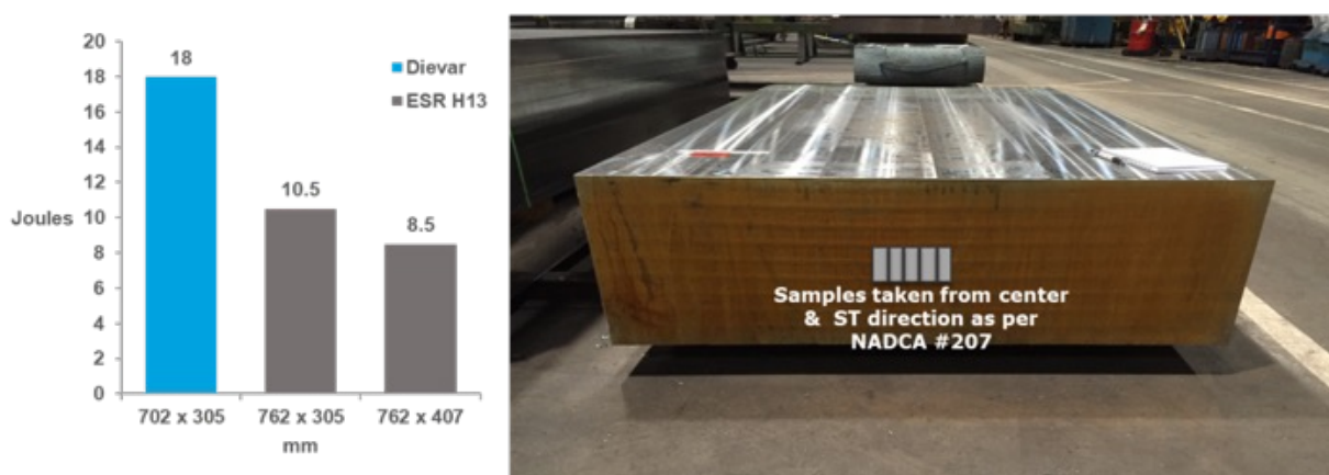
Figure 6 clearly shows Uddeholm Dievar is tougher at higher hardness to premium H13
