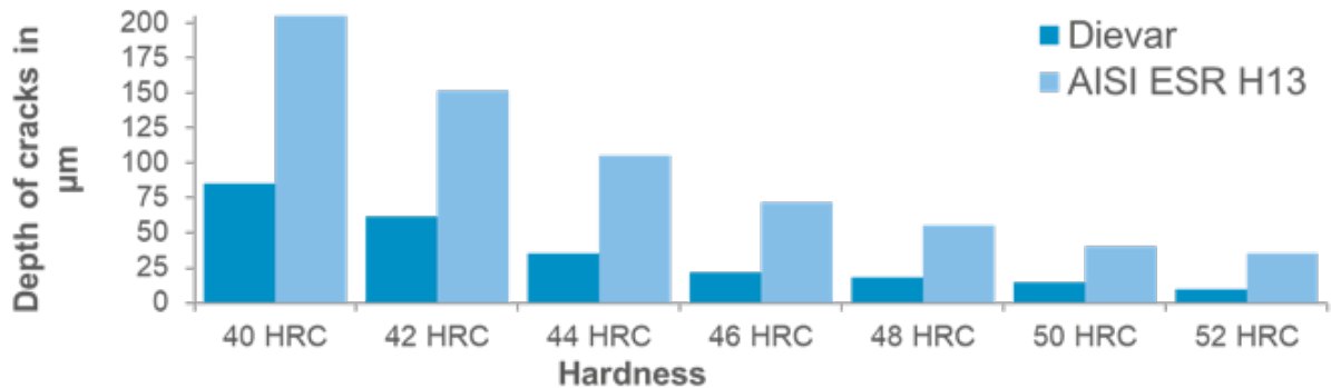
Figure 5 clearly illustrates that Uddeholm Dievar has far superior resistance to heat checking cracks over premium H13
