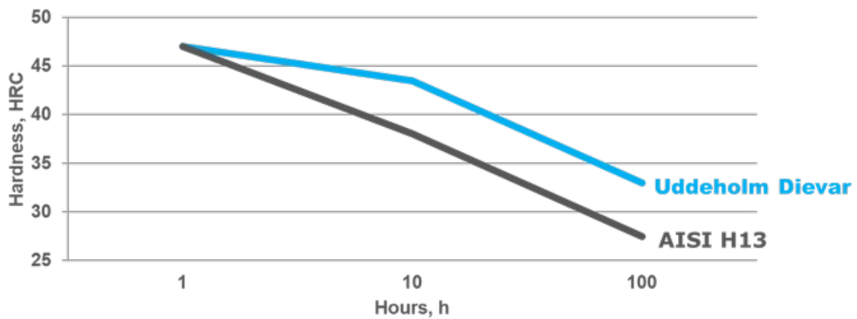
Figure 7 shows just one of the multiple advantages of Dievar chemistry over H13 to fight heat checking, superior temper back resistance
