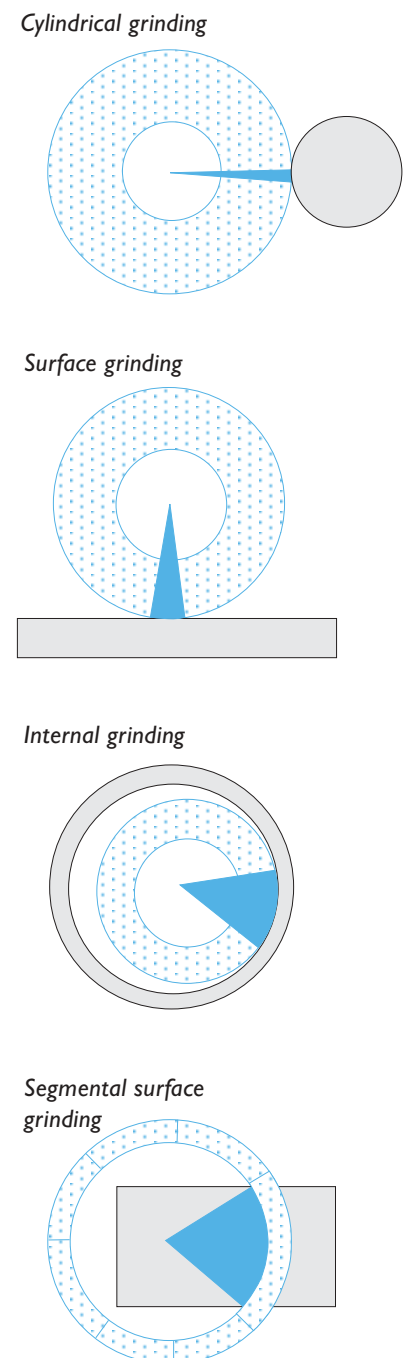
Figure 4. Differences in contact length for different grinding operations.
