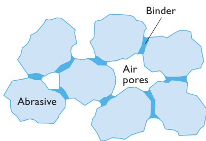
Figure 1. The arrangement and proportions of abrasives grains, air pores and bond bridges (made up of binder) determine grinding wheel characteristics.
