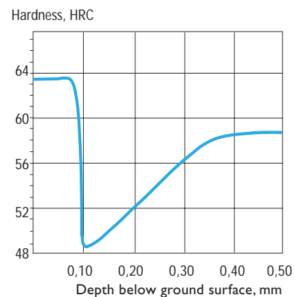
Figure 7. Hardness profile through the surface layer of an incorrectly ground tool.
