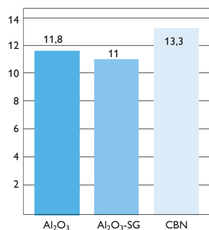
Stock removal rate mm^3/s
