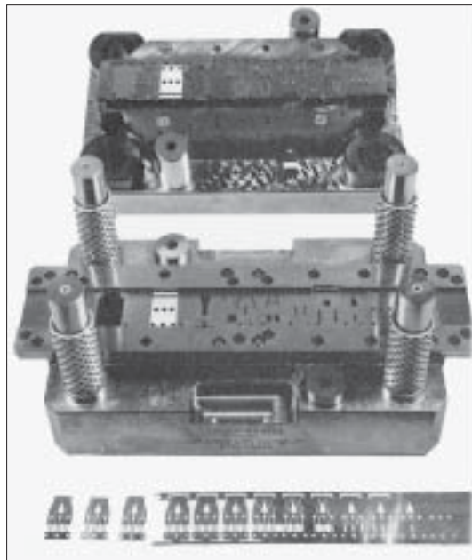
Progressive die made of Uddeholm Sverker 21. Long run tooling for blanking of parts in thin sheets.
