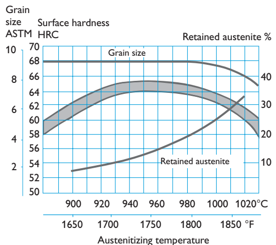
HARDNESS AS A FUNCTION OF HARDENING TEMPERATURE
