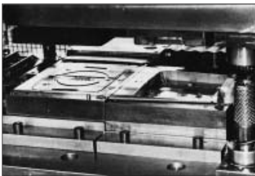
This tool was made from Uddehøm Rigor. 3 million parts were manufactured before the tool was reground.
